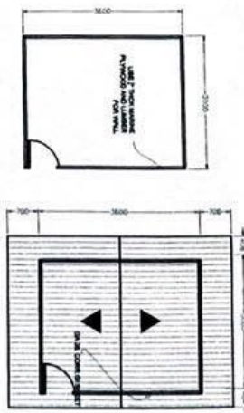
TEMPORARY FACILITY PLAN
